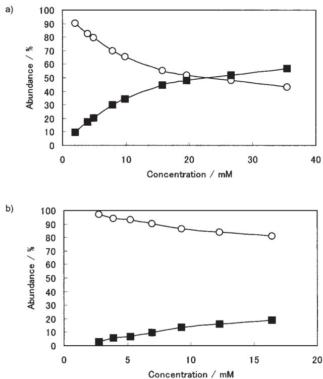
Fig. 8. The abundance of complexes (a) CL3 and (b) CL2 under several concentration conditions in \text{CH}_2\text{Cl}_2 . The abundance of the mononuclear complex and the dinuclear copper(I) complex, are marked with a white circle and a black square, respectively.
