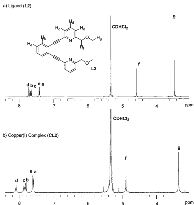
Fig. 1. The ^1\text{H} NMR spectra (400 MHz, \text{CD}_2\text{Cl}_2 ) of (a) the ligand ( L2 ) and (b) the copper(I) complex ( CL2 ).
