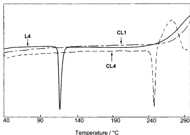
Fig. 6. DSC traces for the thermal cyclization of L4 , CL1 , and CL4 .
