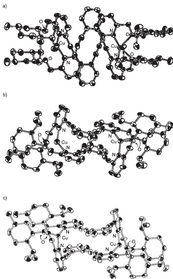
Fig. 5. ORTEP representations of CL4 and CL5 (a) from a top view of CL4 , (b) from a side view of CL4 , and (c) from a side view of CL5 . Counter ions and hydrogen atoms are omitted for clarity.
