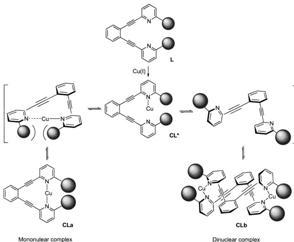
Scheme 3. A proposed mechanism for the self-assembly of the copper(I) complexes (CLa and CLb) in this study.
