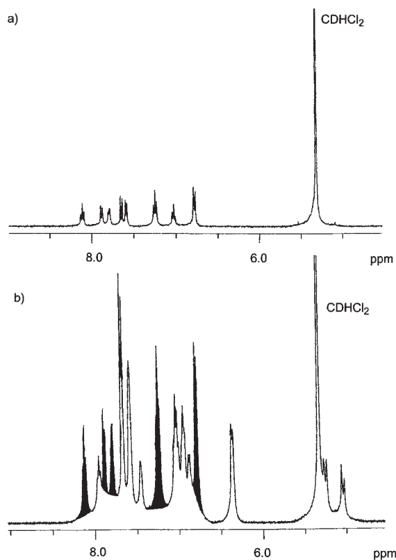
Fig. 7. The ^1\text{H} NMR spectra of CL3 (a) at a dilute concentration (0.98 mM) and (b) at a higher concentration (16 mM).
