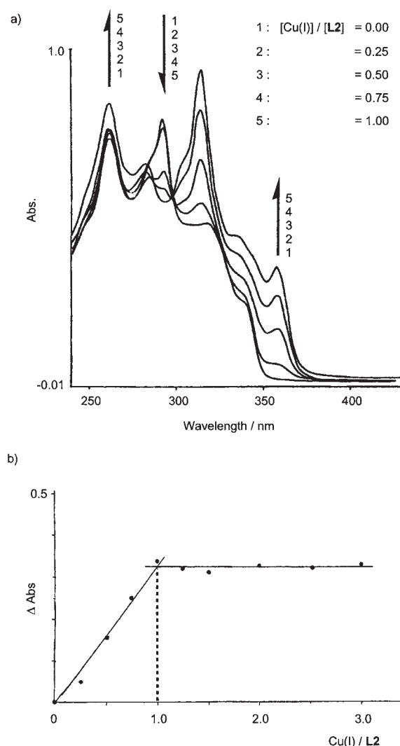
Fig. 2. (a) Spectrophotometric titration of L2 with \text{Cu}(\text{CH}_3\text{CN})_4\text{PF}_6 in \text{CH}_2\text{Cl}_2 . (b) The changes in absorbance analyzed by the mole ratio methods at 358 nm.
