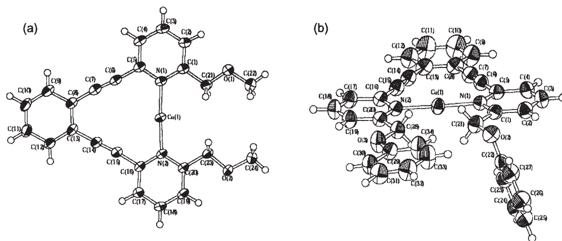
Fig. 4. ORTEP representations of (a) CL2' and (b) CL3 . Counter ions are omitted for clarity.
