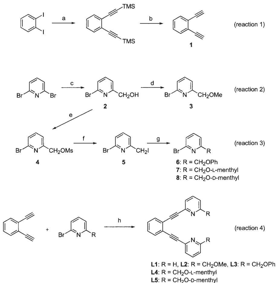
Scheme 1. Preparation of the ligands ( L1–L5 ). Reagents and conditions: (a) TMSacetylene, PdCl 2 (PPh 3 ) 2 , CuI, piperidine, rt, 95%. (b) TBAF, THF–H 2 O, 0 °C to rt, 83%. (c) (1) n -BuLi, THF, –78 °C, (2) DMF, THF, –78 °C, (3) NaBH 4 , THF, 0 °C, 87%. (d) (1) NaH, THF, 0 °C, (2) MeI, THF, 0 °C, 97%. (e) MsCl, Et 3 N, DMAP, THF, –40 °C, 95%. (f) NaI, acetone, 60 °C, 98%. (g) PhONa, THF, 0 °C, 93% (for 6 ), sodium L-menthoxide, THF, 0 °C, 99% (for 7 ), or sodium D-menthoxide, THF, 0 °C, 94% (for 8 ). (h) Pd(PPh 3 ) 4 , Et 2 NH, 80 °C, 72% (for L1 ), 92% (for L2 ), 95% (for L3 ), 68% (for L4 ), and 72% (for L5 ).
