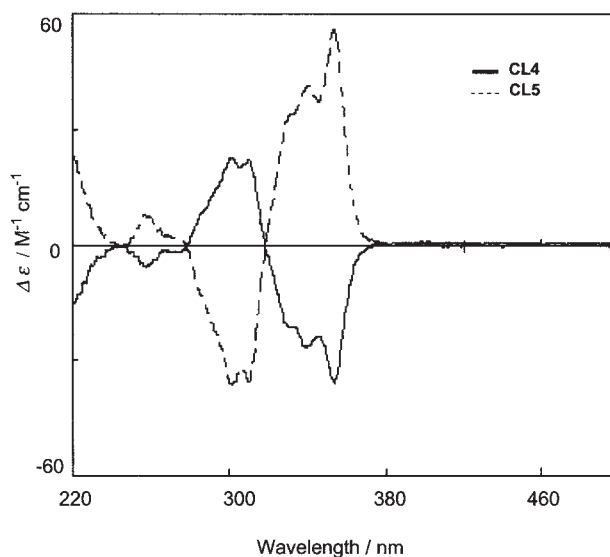
Fig. 3. CD spectra of CL4 and CL5 in chloroform.
